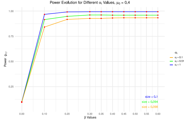
Fig. 9. g_{f,1}^* , encompassing.
