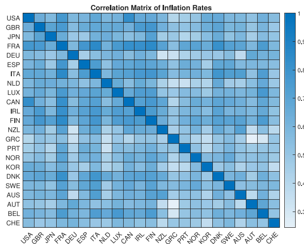
Fig. 14. Correlation heatmap.
