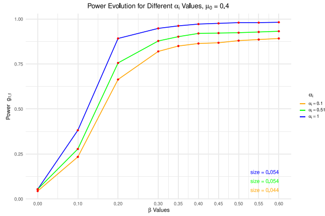
Fig. 1. g_{f,1}^* , encompassing.
