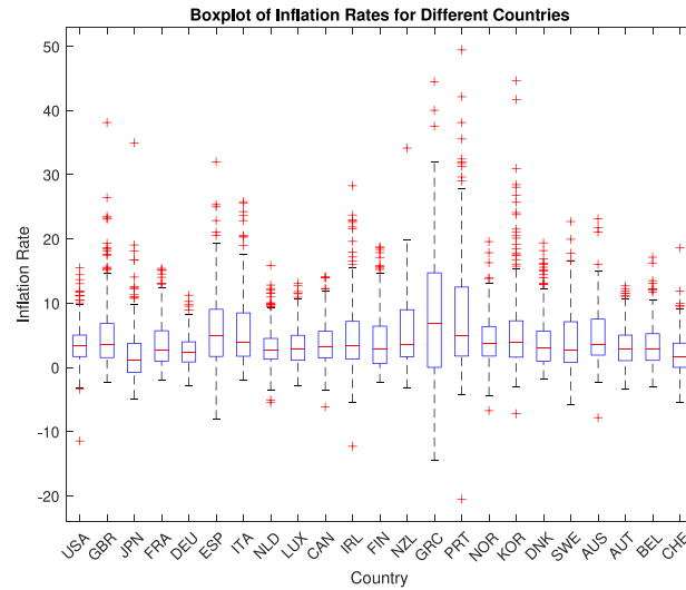
Fig. 13. Inflation boxplot.
